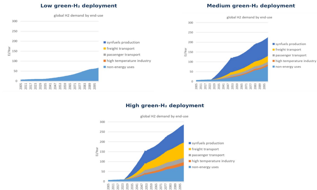
Figure 6. Global H 2 demand by end use in the low-, medium- and high-H 2 deployment scenarios
